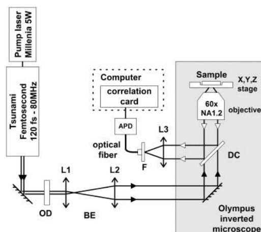
FIGURE 1 Diagram of the experimental two-photon excitation FCS setup. (OD) optical density filter; (BE) beam expander made of two convergent lenses (L1/L2); (DC) dichroic beamsplitter, (F) BG39 filter; (APD) avalanche photodiode.
